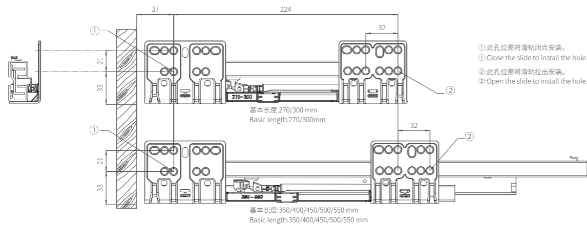
滑轨安装尺寸 Installation size of slide
