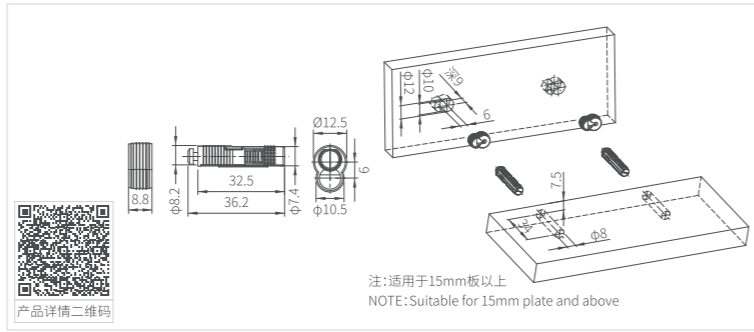
MK-TMBT-31-01-28 33#透明层板托 MK-TMBT-31-01-28 Transparent Shelf Support
