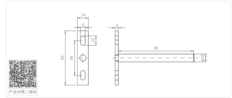
MK-GH-GBT-10-100 Ø10*100一字隐藏隔板膨胀支撑架 MK-GH-GBT-10-100 Ø10*100 Shelf support
