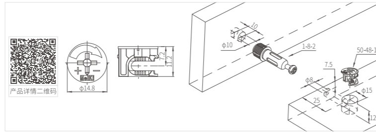
MKCAM-ZA-50-53-27 锌合金偏心轮 MKCAM-ZA-50-53-27 Zinc alloy eccentric cam
