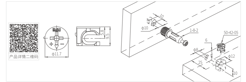
MKCAM-ZA-50-00-03 锌合金偏心轮 MKCAM-ZA-50-00-03 Zinc alloy eccentric cam
