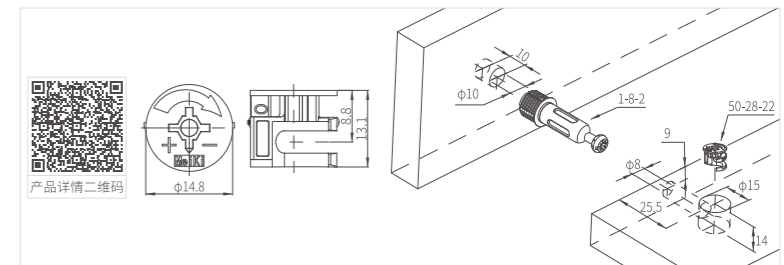
MKCAM-ZA-50-13-31 锌合金偏心轮 MKCAM-ZA-50-13-31 Zinc alloy eccentric cam
