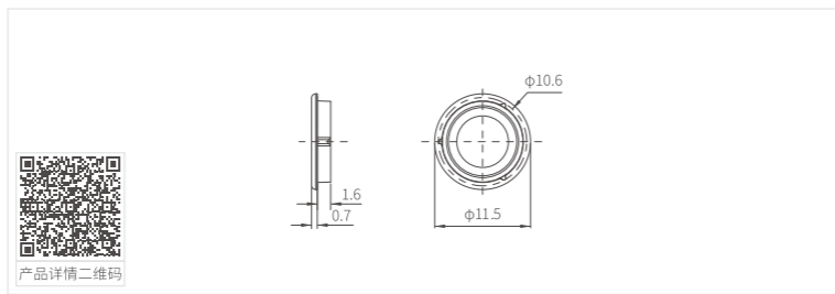
MK-KG-32-01-09 3# 12下沉式塑料盖 MK-KG-32-01-09 3# 12 Countersunk plastic cover
